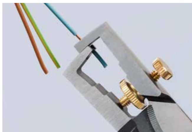
Length marking: visual markings provide support during repeated stripping of wire in standard lengths (11 and 16 mm)
