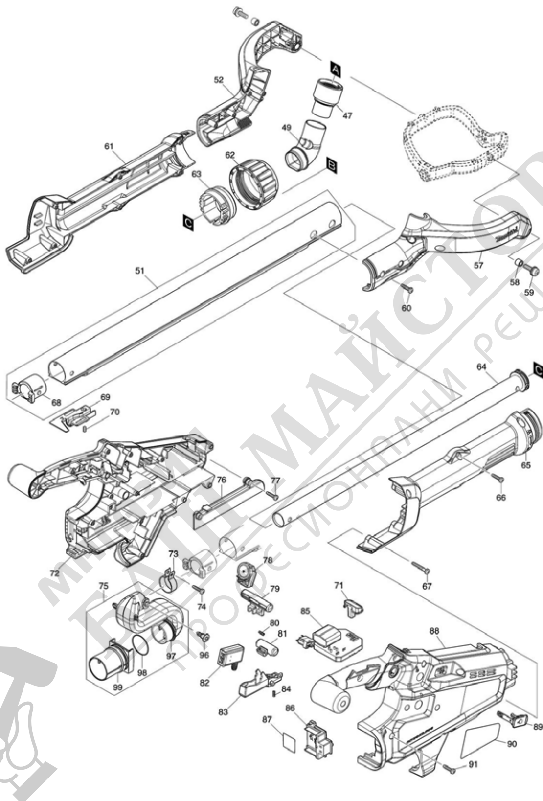
Model No.DSL801 225MM CORDLESS DRYWALL SANDER
