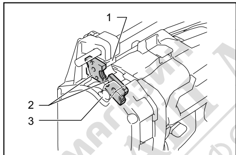
► 1. Stationary mount 2. Cutting die 3. Movable mount
