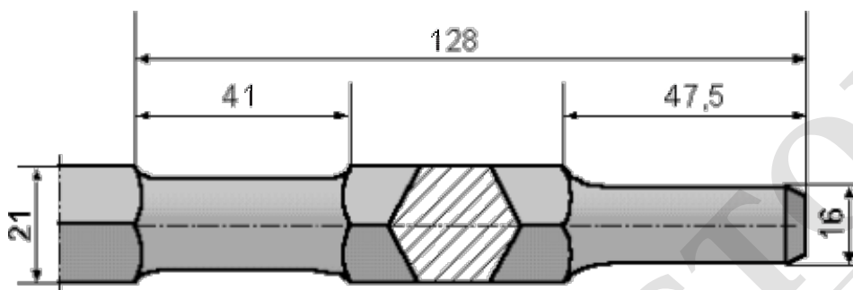
Flat Cold Chisel
