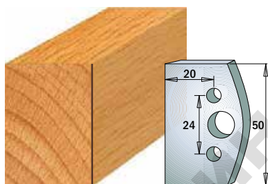
Pair of knives 690.500 Pair of limiters 691.500
