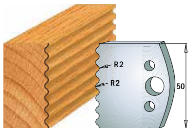
Pair of knives 690.552 Pair of limiters 691.552
