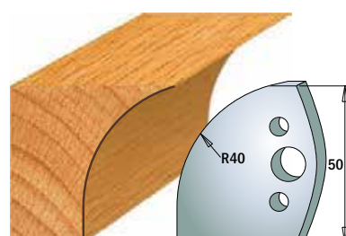
Pair of knives 690.565 Pair of limiters 691.565
