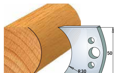
Pair of knives 690.547 Pair of limiters 691.547
