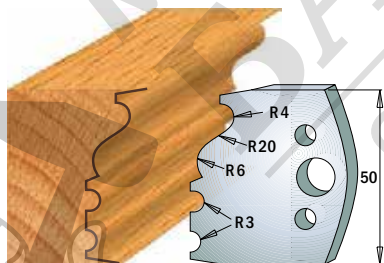
Pair of knives 690.513 Pair of limiters 691.513
