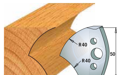
Pair of knives 690.550 Pair of limiters 691.550
