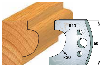
Pair of knives 690.504 Pair of limiters 691.504
