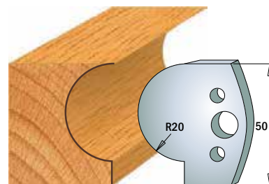
Pair of knives 690.562 Pair of limiters 691.562
