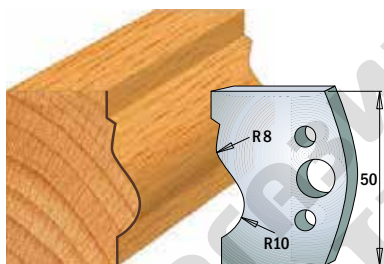
Pair of knives 690.510 Pair of limiters 691.510
