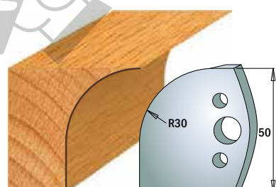
Pair of knives 690.563 Pair of limiters 691.563
