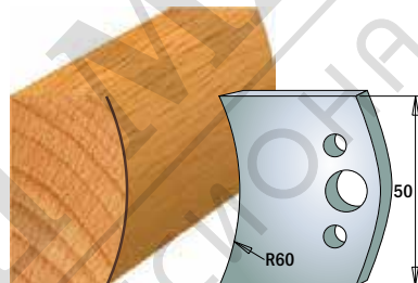
Pair of knives 690.573 Pair of limiters 691.573
