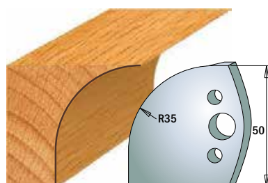
Pair of knives 690.564 Pair of limiters 691.564
