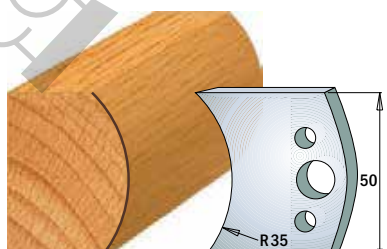
Pair of knives 690.548 Pair of limiters 691.548
