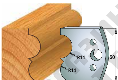
Pair of knives 690.572 Pair of limiters 691.572
