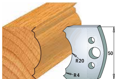
Pair of knives 690.507 Pair of limiters 691.507
