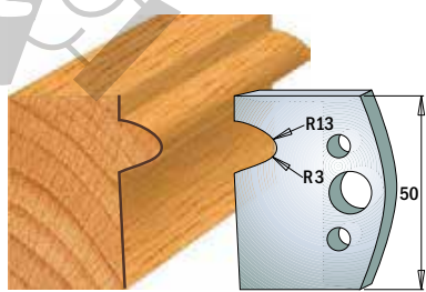
Pair of knives 690.516 Pair of limiters 691.516
