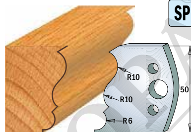
Pair of knives 690.506 Pair of limiters 691.506
