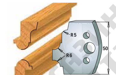
Pair of knives 690.542 Pair of limiters 691.542
