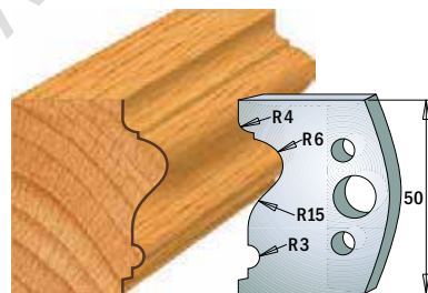
Pair of knives 690.512 Pair of limiters 691.512
