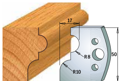
Pair of knives 690.551 Pair of limiters 691.551
