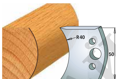
Pair of knives 690.555 Pair of limiters 691.555
