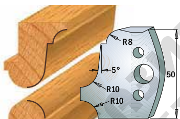
Pair of knives 690.557 Pair of limiters 691.557
