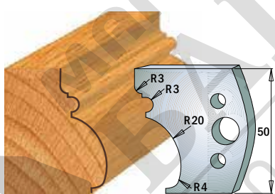
Pair of knives 690.501 Pair of limiters 691.501
