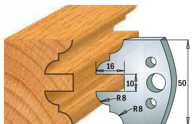
Pair of knives 690.523 Pair of limiters 691.523
