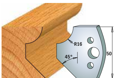
Pair of knives 690.569 Pair of limiters 691.569
