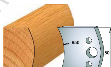
Pair of knives 690.559 Pair of limiters 691.559
