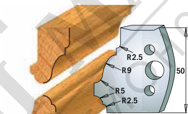
Pair of knives 690.558 Pair of limiters 691.558
