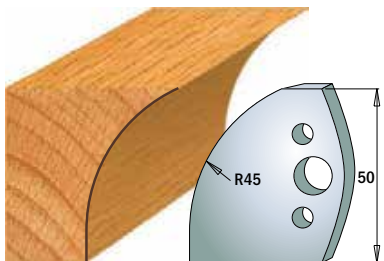
Pair of knives 690.566 Pair of limiters 691.566
