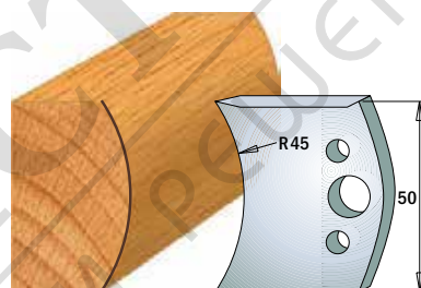
Pair of knives 690.556 Pair of limiters 691.556
