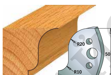
Pair of knives 690.570 Pair of limiters 691.570
