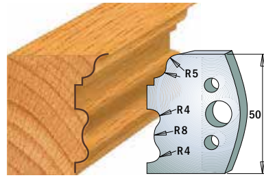
Pair of knives 690.515 Pair of limiters 691.515
