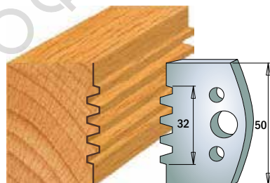
Pair of knives 690.576 Pair of limiters 691.576
