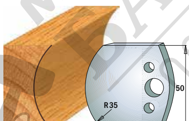
Pair of knives 690.545 Pair of limiters 691.545
