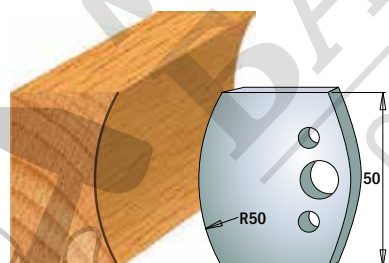
Pair of knives 690.560 Pair of limiters 691.560
