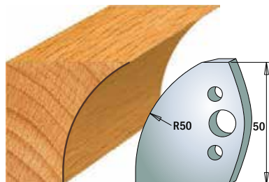
Pair of knives 690.567 Pair of limiters 691.567
