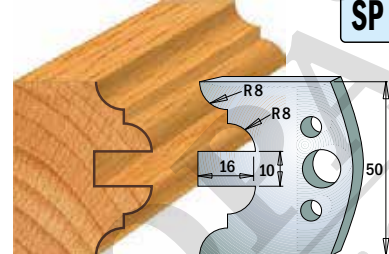
Pair of knives 690.522 Pair of limiters 691.522
