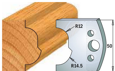
Pair of knives 690.519 Pair of limiters 691.519
