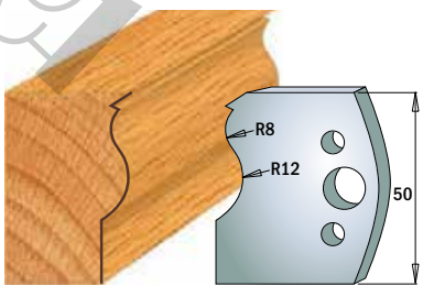
Pair of knives 690.578 Pair of limiters 691.578
