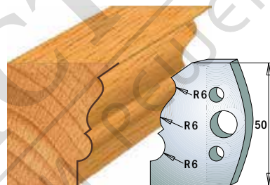
Pair of knives 690.509 Pair of limiters 691.509
