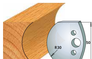
Pair of knives 690.544 Pair of limiters 691.544
