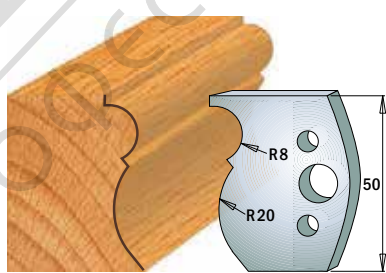
Pair of knives 690.502 Pair of limiters 691.502
