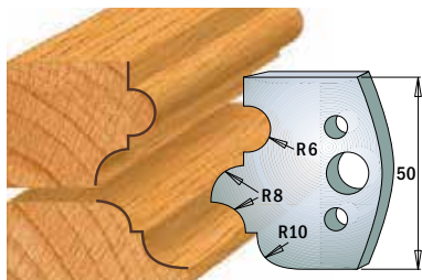
Pair of knives 690.520 Pair of limiters 691.520
