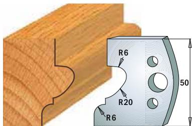
Pair of knives 690.505 Pair of limiters 691.505
