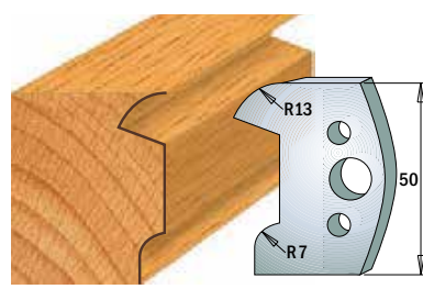
Pair of knives 690.518 Pair of limiters 691.518
