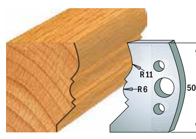
Pair of knives 690.503 Pair of limiters 691.503
