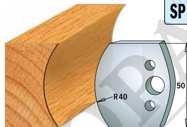
Pair of knives 690.553 Pair of limiters 691.553
