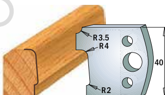
Pair of knives 690.130 Pair of limiters 691.130
