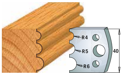
Pair of knives 690.090 Pair of limiters 691.090
