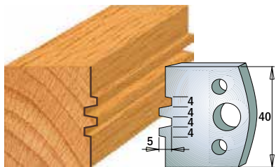
Pair of knives 690.075 Pair of limiters 691.075
