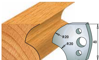
Pair of knives 690.120 Pair of limiters 691.120
