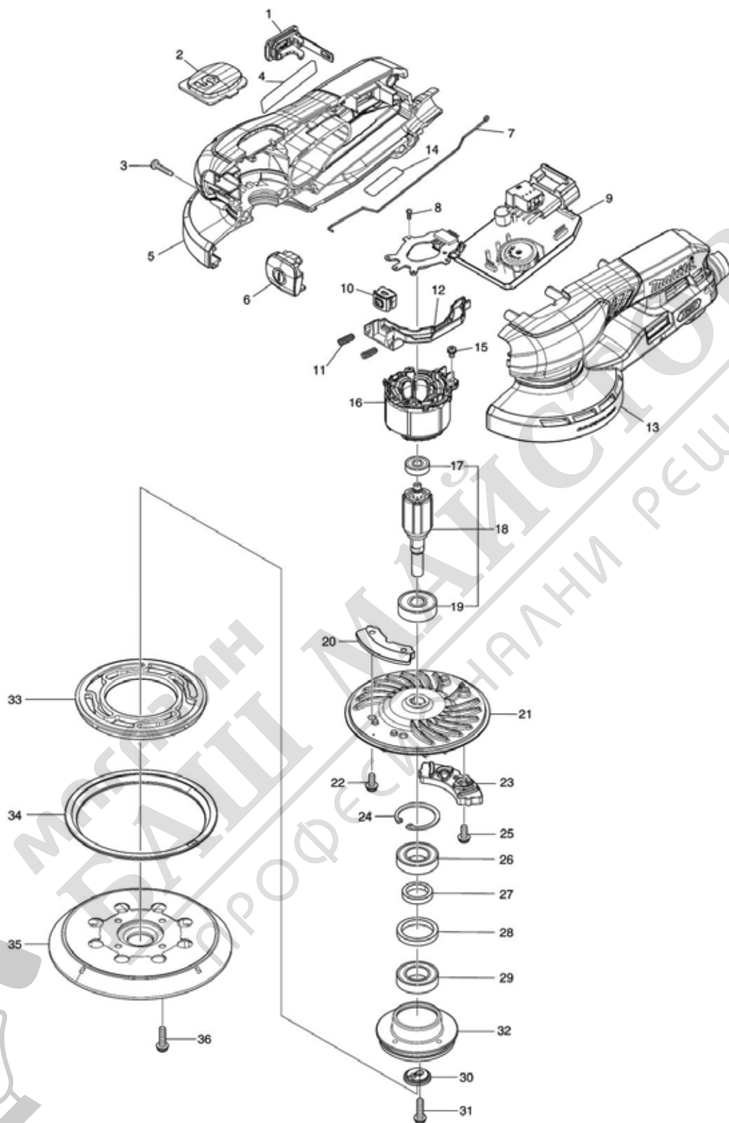
Model No.BO001CG BP RANDOM ORBIT SANDER
